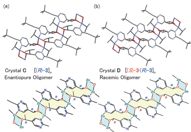
Figure 2. Single-crystal X-ray structures and simplified schematic drawing of alkoxide oligomer crystallized with 1–2 equiv i\text{Pr}_2\text{Zn} . a) Enantiopure alkoxide oligomer crystal C . b) Racemic alkoxide oligomer crystal D .
